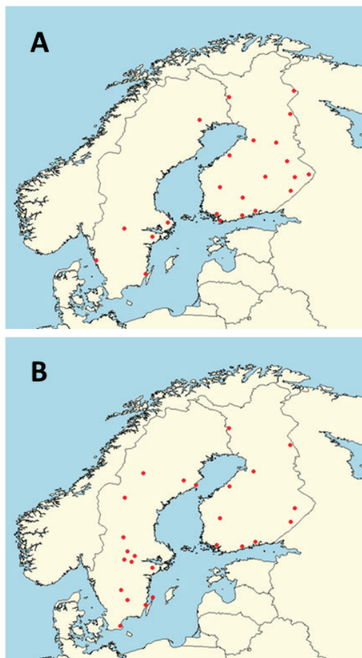
Fig 3. Maps over sites where phenological observations used in this study were made to determine the dates for budburst ( A ) and the dates for the start of autumn coloration ( B ) for Birch ( Betula pendula and B. pubescens ) in Sweden and Finland. Source for Finnish data: Dr Eero Kubin, Finnish Forest Research Institute, Muhos Research Unit. Source for Swedish data: Dr Kjell Bolmgren.
