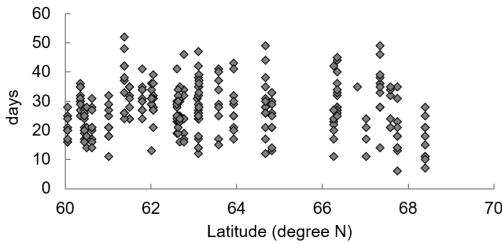
Fig 7. Estimate of the number of days between first observations of budburst and fully expanded leaves for Birch at sites with different latitudes in Finland 1997–2006. The value used in the Mapping Manual (UNECE 2017) for f_{phen1} for deciduous trees is 20 days. The maps with information about the state of budburst were obtained from Eero Kubin, Finnish Forest Research Institute, Muhos Research Unit.
