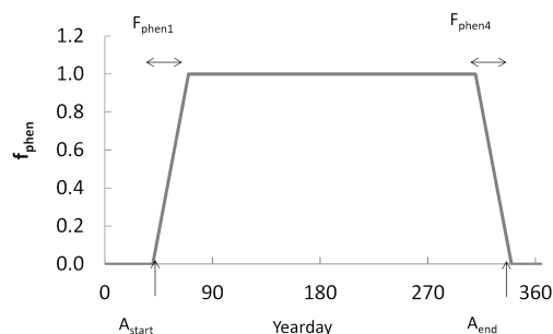
Fig 1. The f_{\text{phen}} function describes how the phenology limits the estimated potential stomatal ozone uptake during \text{O}_3\text{AP} during different parts of the year for northern and central European tree species. At f_{\text{phen}} = 1 the phenology does not limit stomatal ozone uptake. The day of year after the winter dormancy period when the \text{O}_3\text{AP} of a certain tree species begins is called " A_{\text{start}} " and the day of year during autumn when \text{O}_3\text{AP} ends is called " A_{\text{end}} ". The duration from f_{\text{phen}} = 0 at " A_{\text{start}} " to reach f_{\text{phen}} = 1 is called f_{\text{phen1}} . The number of days it takes from f_{\text{phen}} = 1 to f_{\text{phen}} = 0 before " A_{\text{end}} " is called f_{\text{phen4}} . The different abbreviations and the figure are simplified from the Mapping Manual (UNECE 2017).
