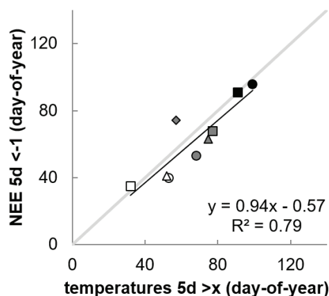
Fig 4. The correlation between the day-of-year for the start of NEE, and the day-of-year for 24h mean air temperatures exceeding the different thresholds for three ICOS sites. On the y-axis is shown the day-of-year when the daytime \text{CO}_2 NEE decreased below -1 \mu\text{mol m}^{-2} \text{s}^{-1} for five consecutive days. On the x-axis is shown the corresponding day-of-year when the 24h air temperatures exceeded a threshold value for five consecutive days. The threshold values were 1.5^\circ\text{C} for the southern sites Hyltemossa (white symbols) and Norunda (grey symbols) and 0^\circ\text{C} for the northern site Svartberget (black symbols). Data were from four different years, 2014 (diamonds), 2015 (circles), 2016 (squares) and 2017 (triangles). The solid grey line shows the 1:1 relationship.
