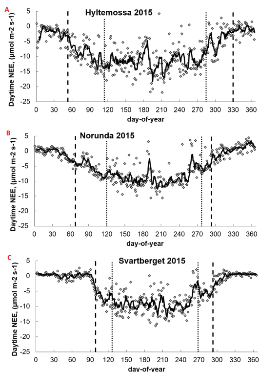
Fig 5. Daily values for Net Ecosystem Exchange of \text{CO}_2 (NEE) as mean values for the middle of the day (10:00–13:59) for the year 2015 for Hyltemossa (A), Norunda (B) and Svartberget (C) plotted versus day-of-year. A solid black line indicates the running five-day mean values. Vertical broken black lines indicate the A_{\text{start}} and A_{\text{end}} estimated with the new method suggested in this study based on 24h mean air temperatures. Vertical dotted black lines indicate the A_{\text{start}} and A_{\text{end}} estimated with the current methods in the Mapping Manual.
