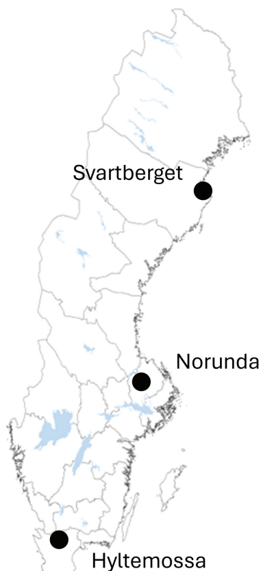
Fig 2. A map showing the three sites in Sweden with micro-meteorological measurements of "Net Ecosystem Exchange", NEE, of CO 2 within ICOS-Sweden ( http://www.icos-sweden.se ) as well as showing the location of the 21 different counties of Sweden, used in the analysis for the agricultural crops. Hyltemossa (56° 10'N, 13° 42'E, 115 m a.s.l.) is positioned in southernmost Sweden, nemoral zone. Svartberget (64°15'N, 19°46'E, 270 m a.s.l.) is positioned in north Sweden, boreal zone. Norunda (60°05'N, 17°29'E, 46 m a.s.l.) is positioned in the transition between the boreal and nemoral zones.
