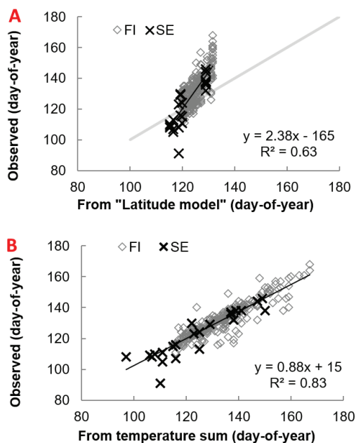
Fig 6. A comparison of the prediction of the time for budburst (day-of-year) for Birch in Sweden and Finland, compared to observed time for budburst, based on the currently used method in the Mapping Manual (UNECE 2017), i.e. the "Latitude model" (A), and based on the method developed in this study, based on the accumulated air temperature sum since 1 January, (B). In the latter model budburst is assumed to occur when the 24h air temperature sum exceed 45 degree-days. The analysis is based on phenology observations from Sweden (SE) and Finland (FI).
