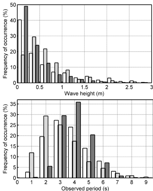
Fig. 2. Frequency of occurrence of different wave heights (above, resolution 0.25 m) and mean periods (below, resolution 1 s) at Vilsandi (white bars), Pakri (light grey bars) and Narva-Jõesuu (dark grey bars).
