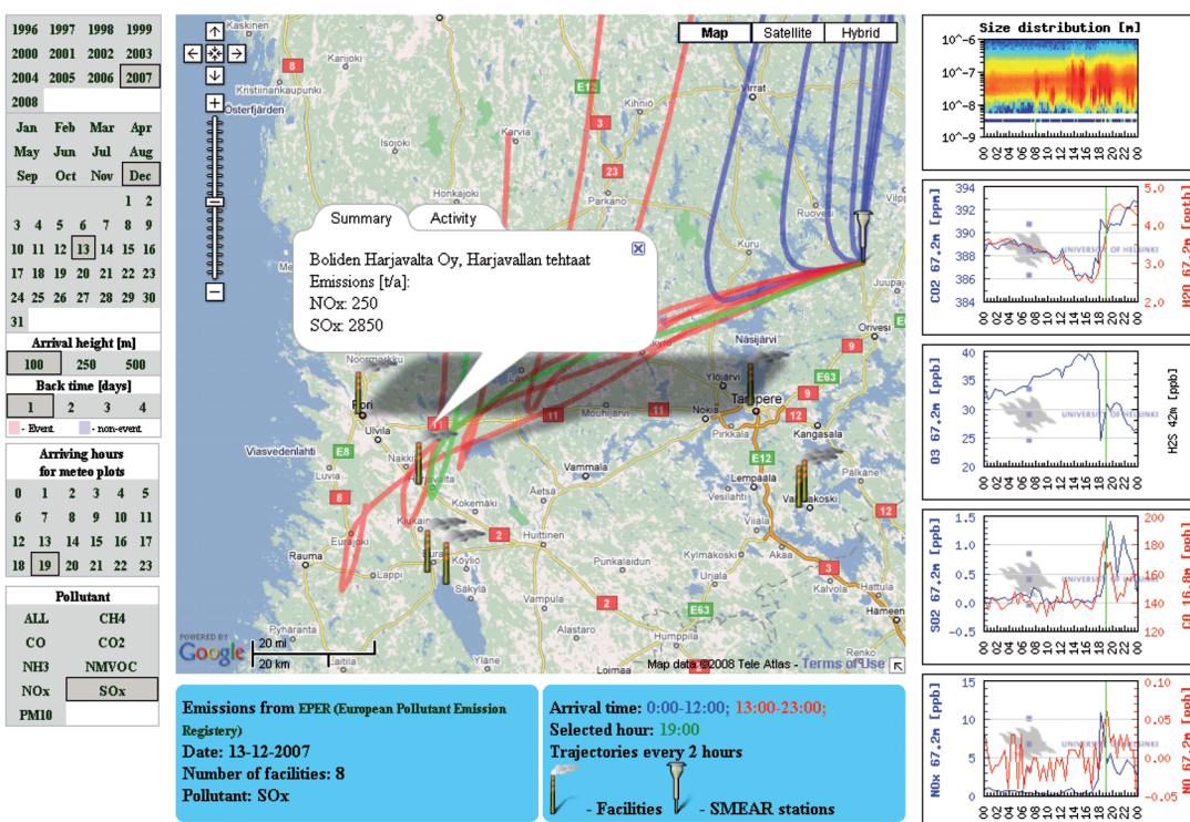
Fig. 5. Screenshot presenting a pollution event in Hyytiälä on 13 December 2007, only SO 2 polluters are shown.
