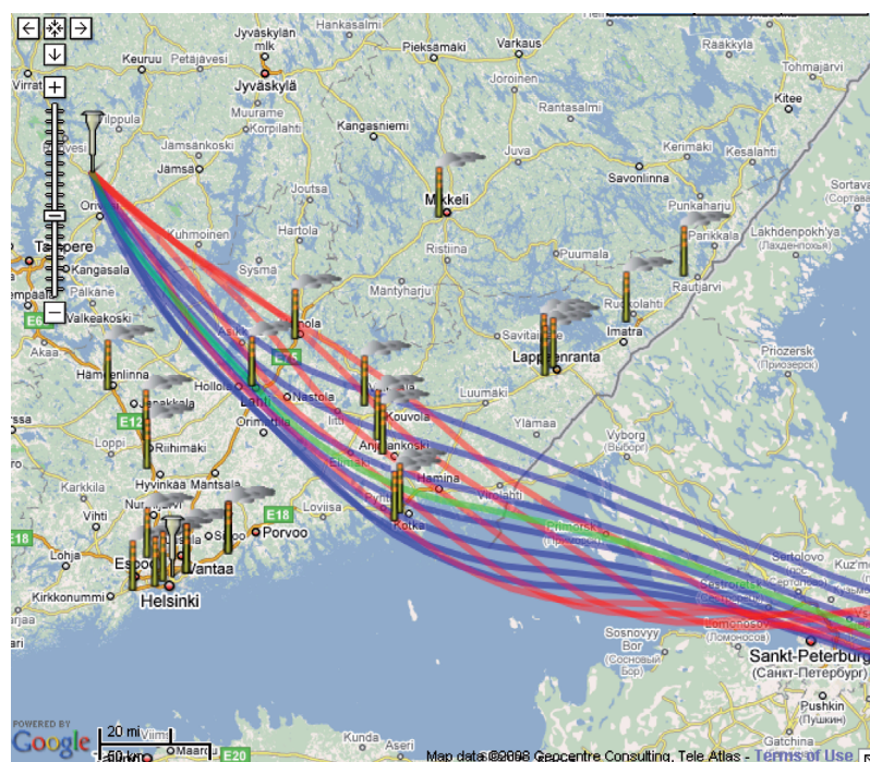
Fig. 8. Screenshot presenting air mass 48-hour back trajectories. Blue lines are before noon trajectories, red lines after-noon trajectories and green line is the trajectory arriving at Hyttiälä at 05:00.
