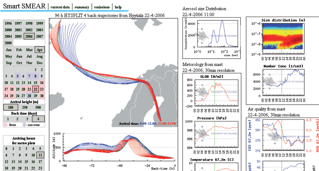
Fig. 4. Screenshot presenting a new-particle formation day, 22 April 2006. Note that the screen shot is not of a full screen.
