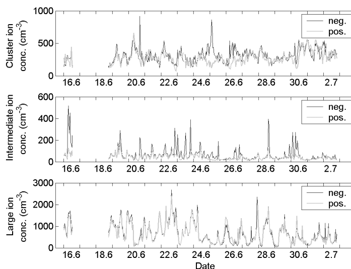
Fig. 2. Hourly-average cluster ion (0.3–1.8 nm), intermediate ion (1.8–7.5 nm) and large ion (7.5–40 nm) concentrations during measurement campaign. The data between 13:00 on 16 June 2004 and 20:00 on 18 June 2004 is not valid because of a failure in the measurement system so the data have been removed from further analysis.
