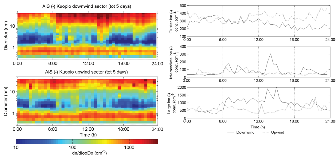
Fig. 6. Diurnal variation of negative ion (left-hand side) size distributions during downwind (top) and upwind condition (bottom), (right-hand side) concentration during downwind (solid line) and upwind condition (dotted line).
