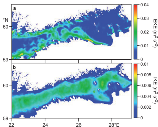
Fig. 5. Maps of simulated (a) eddy kinetic energy and (b) inertial oscillation kinetic energy in the surface layer of the Gulf.
