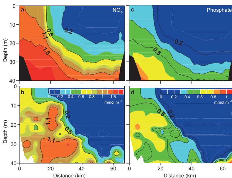
Fig. 7. Comparison of (a, c) simulated and (b, d) measured \text{NO}_x and \text{PO}_4 concentrations along the transect between Tallinn and Helsinki on 8 August. The values on the x-axis denote the distance from the southernmost sampling station. Separate colour scales for \text{NO}_x and \text{PO}_4 concentrations were used.
