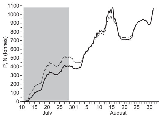
Fig. 8. Temporal course of total content of phosphorus (thin line) and nitrogen (bold line) introduced to the upper 10-m layer due to upwelling events along the northern (shaded area) and southern coasts during the simulation period in the Gulf of Finland.
