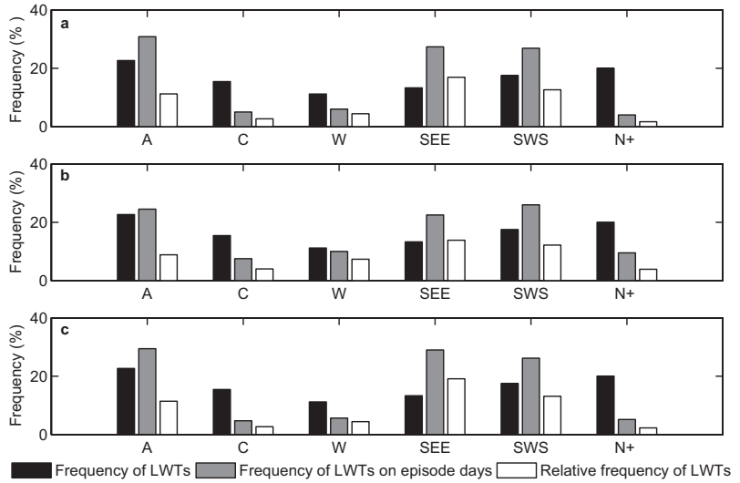
Fig. 4. Comparison of the frequencies for daily LWTs at (a) Rörvik/Råö, (b) Norra Kvill and (c) Vavihill from April to August over the period of 1990–2005. The black bars represent the frequencies of LWTs based on all days, the grey bars represent the frequencies of LWTs based on the episode days and the white bars represent the relative frequencies of episode days associated with a certain LWT.
